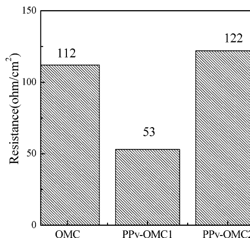
Figure 6. Interfacial electrical resistance of pristine OMC and PPy-OMCs after doping with LiClO_4 .
